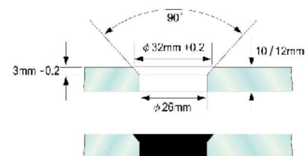
Countersunk hole type (C)
