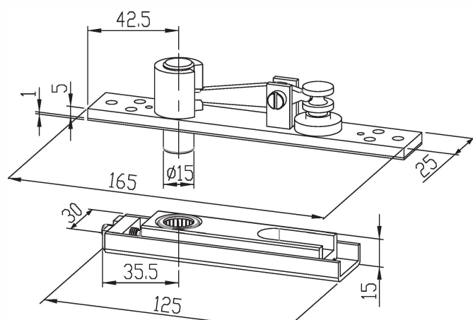
9180 Adjustable top centre Ø15mm pin
