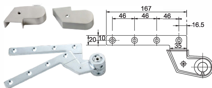
9149TC Offset top centre
