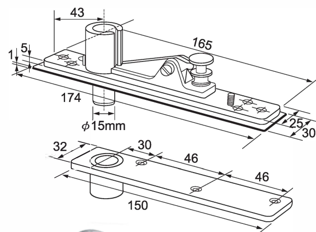
9118/9 Top centre Ø15mm pin
