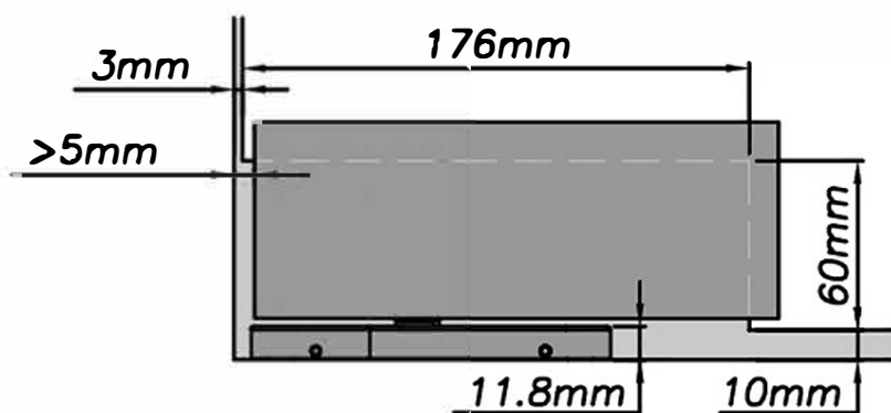
Glass Cutout(HGT-100/HGT-100H):
