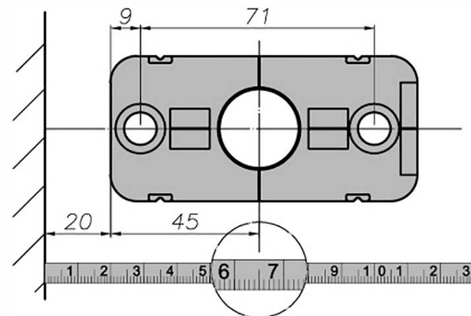
Glass Cutout(HGT-100/HGT-100H):
