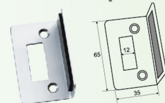
LLP-403 Keeper Plate
