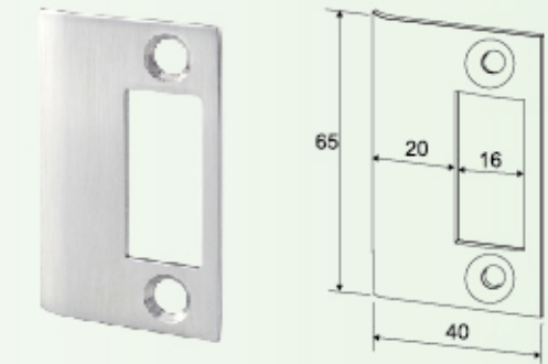
LLP-401 Strike Plate
