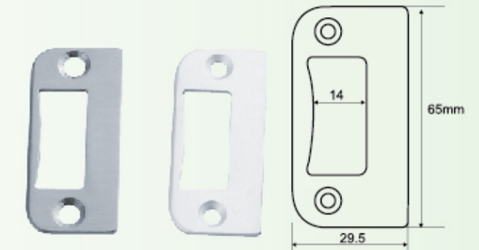
LLP-402 Strike Plate
