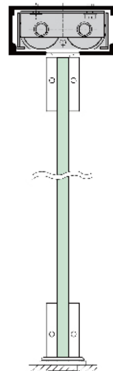
Double action tempered glass door
